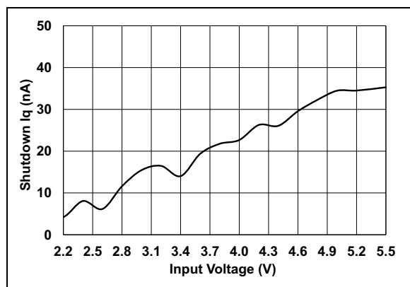
FIGURE 2-8: Shutdown Quiescent Current, I_{QSHDN} , vs. V_{IN} ( EN = GND ).
