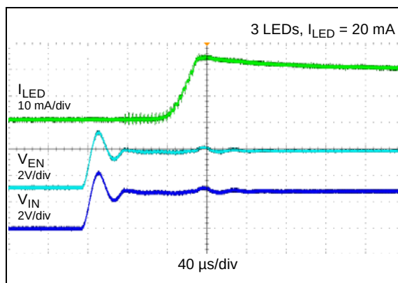
FIGURE 2-11: Start-Up When V_{IN} = V_{ENABLE} .
