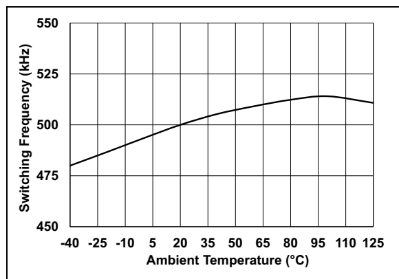
FIGURE 2-9: Switching Frequency, f_{SW} , vs. Ambient Temperature.
