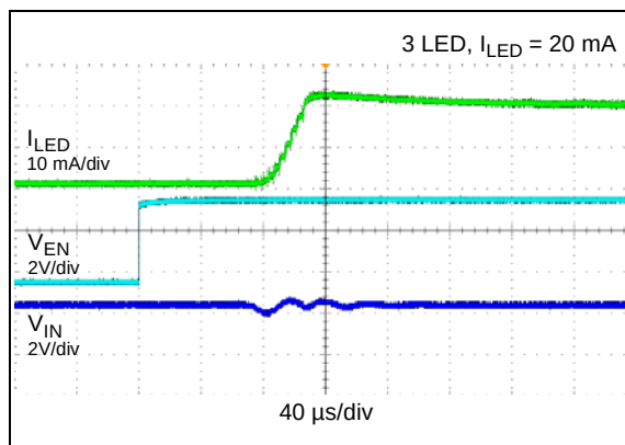
FIGURE 2-12: Start-Up After Enable.
