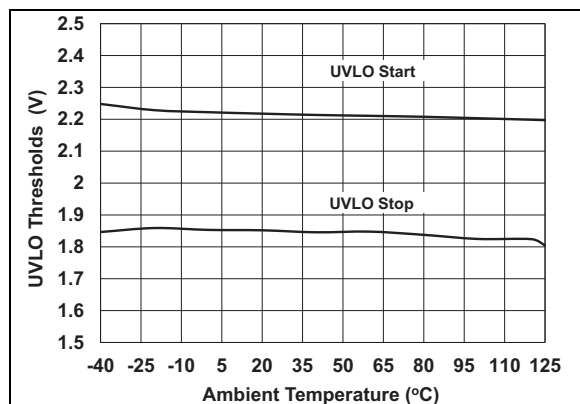
FIGURE 2-7: Undervoltage Lockout (UVLO) vs. Ambient Temperature.
